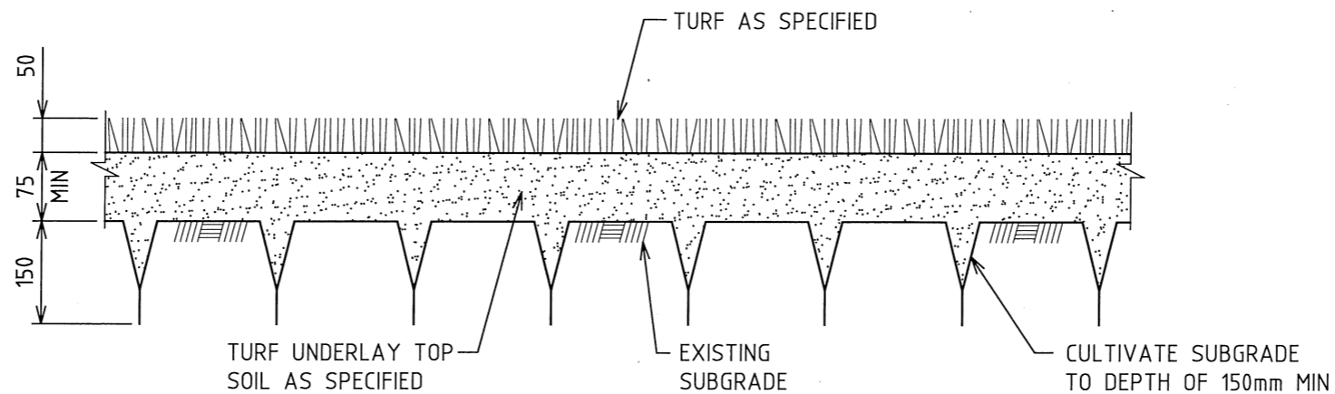
SECTION TURF - SOIL PROFILE AND INSTALLATION DETAILS SCALE 1:10
